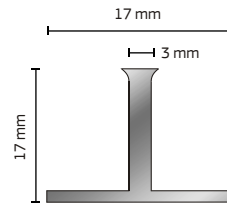
QMT17A (Aluminium) QMT17B (Brass)
