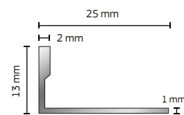
QMF13A (Aluminium) QMF13B (Brass) QMF13S (Stainless Steel)
