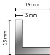
QM6A (Aluminium) QM6S (Stainless Steel)
