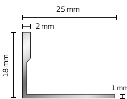
QMF18A (Aluminium) QMF18B (Brass)
