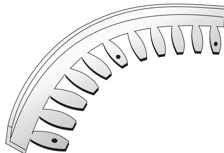
QMT17A (Aluminium) QMT17B (Brass)
