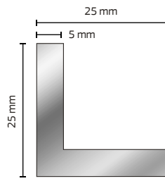
QM3A (Aluminium) QM3B (Brass)
