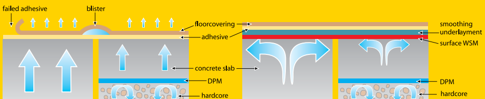
Floorcovering traps moisture release causing blisters or damage to adhesive layer allowing floorcovering to lift
