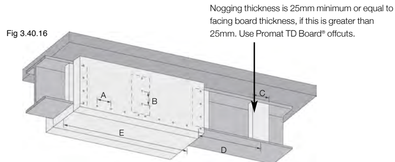
3-sided box using adhesive noggings
