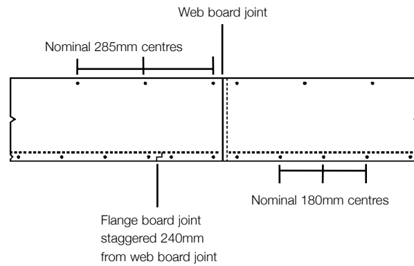
Fixing centres in relation to board joints for beams – Side elevation
